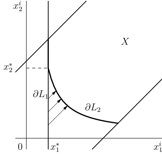
Figure 4: Illustration of the argument supporting Lemma 1.
