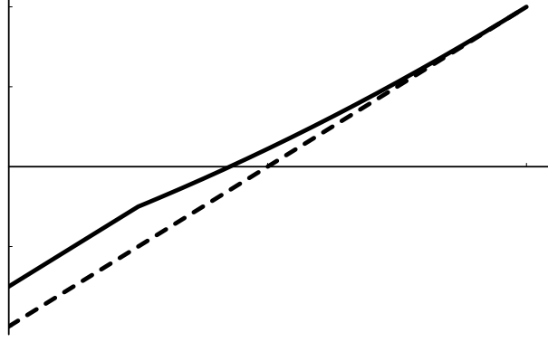
Figure 6: Comparison of functions m_{st}^*(x_1) and m_{dyn}^*(x_1) in the ordered limit.
