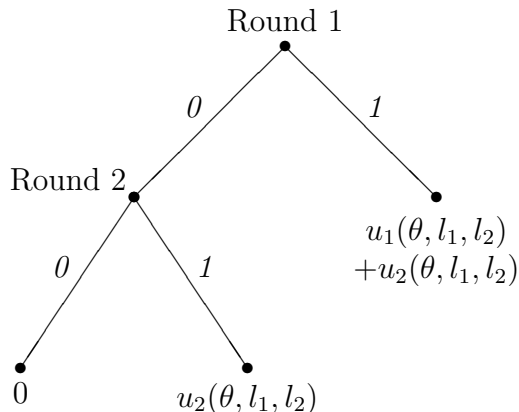
Figure 3: Variant of the dynamic game in which players can delay investment.
